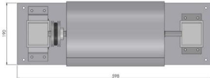
Rotating Drum Collector
